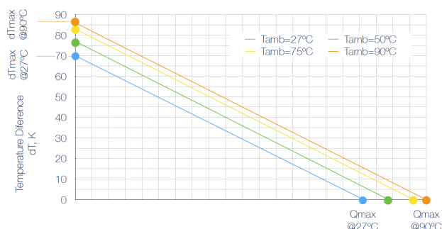
Fig. 2 - Single-stage TEC dT_{max} and Q_{max} example
