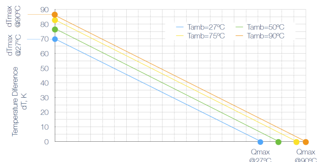
Fig. 2 - Single-stage TEC dT_{max} and Q_{max} example
